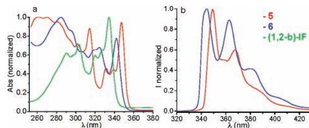
Figure 4. (a) UV-vis spectra of 5 , 6 , and (1,2- b )-IF in CH 2 Cl 2 . (b) Emission spectra of 5 and 6 in cyclohexane (10 -6 M).
