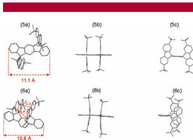
Figure 2. Molecular structure of 5 and 6 . Top (a) and side views (b and c), from single-crystal X-ray data.
